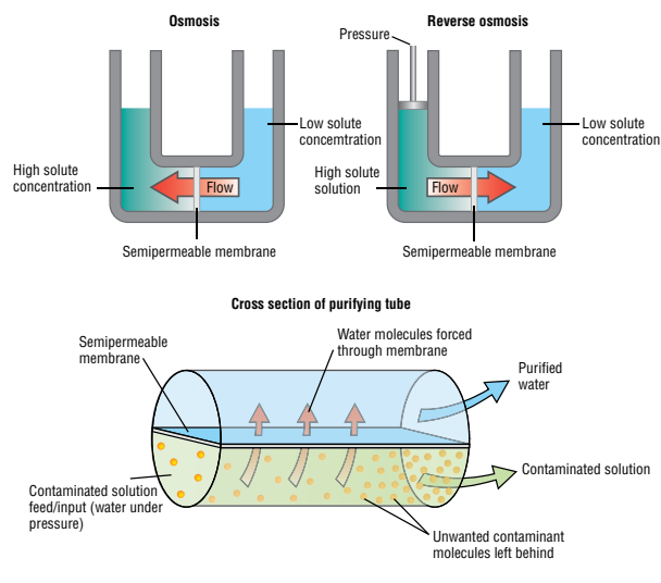
Figure 2. How reverse osmosis works
