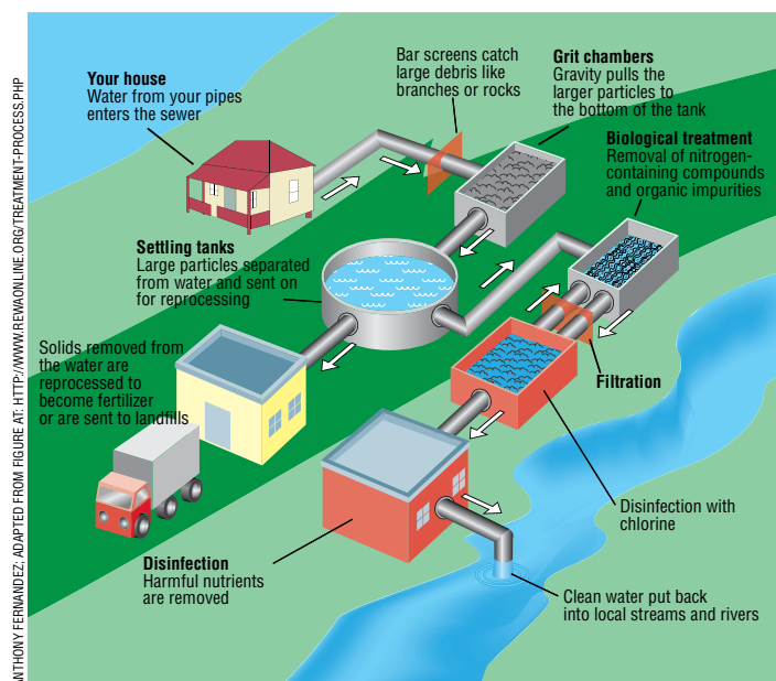
Figure 1. The various steps of the wastewater treatment process
